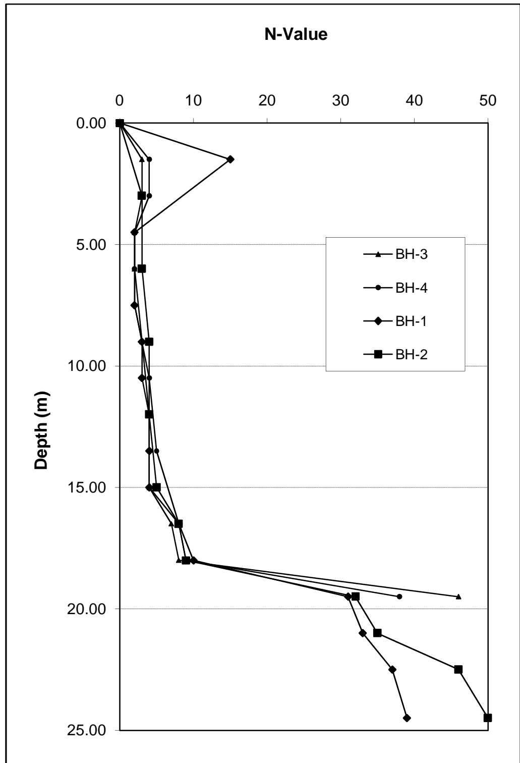
Figure 3A: Distribution of Field N-Value with Depth
